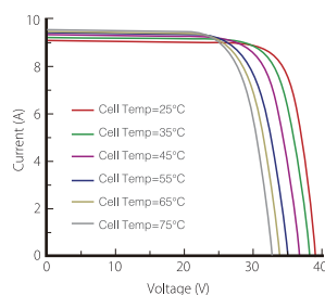
Current-Voltage Curve (LR6-60BK-290M)
